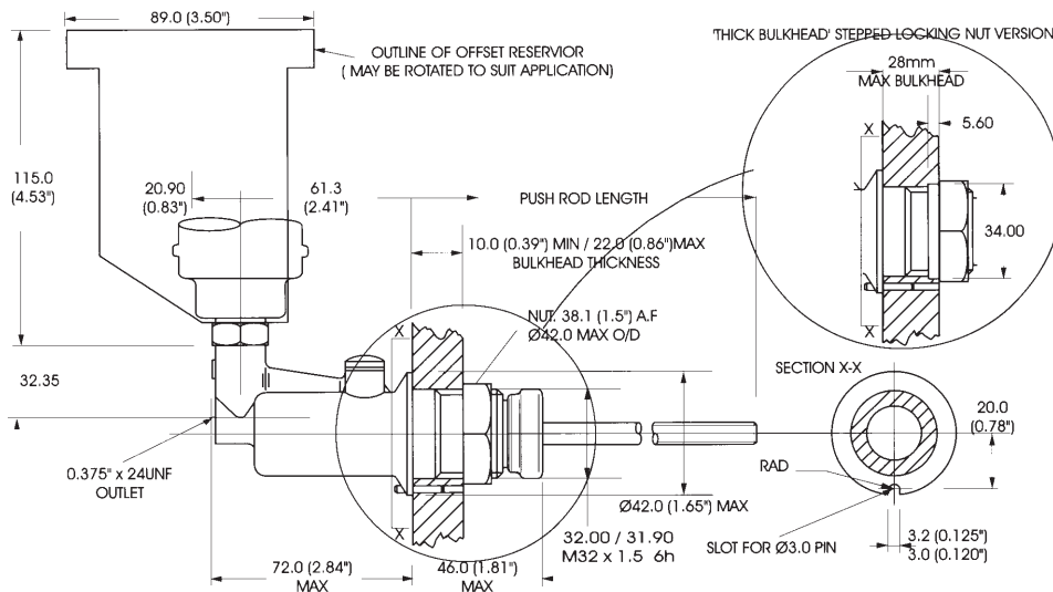
Installation Dimension Drawing - CP4400 Master Cylinder
